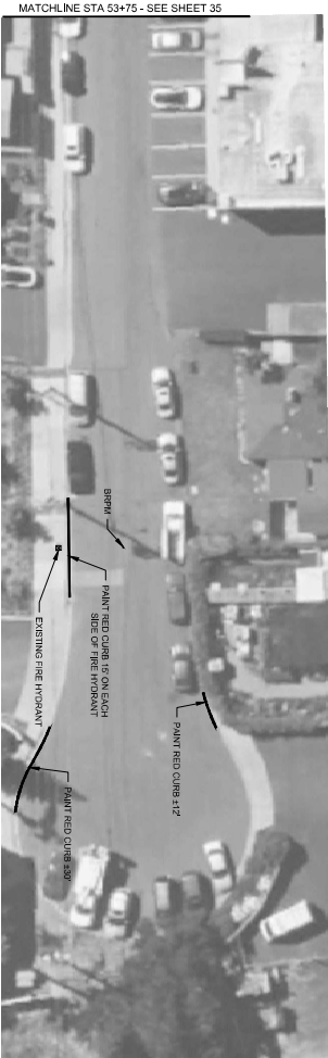
SOUTH FAIRVIEW AVENUE - STRIPING LAYOUT
