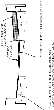
TYPICAL SECTION NO. 3
