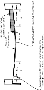
TYPICAL SECTION NO. 3 NTS
