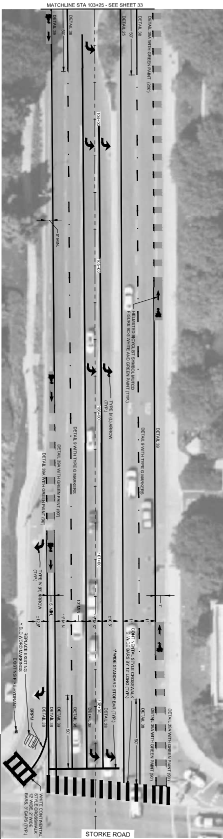
HOLLISTER AVENUE - STRIPING LAYOUT
