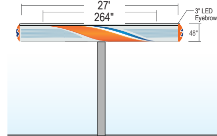
ELEVATION D: ILLUMINATED
